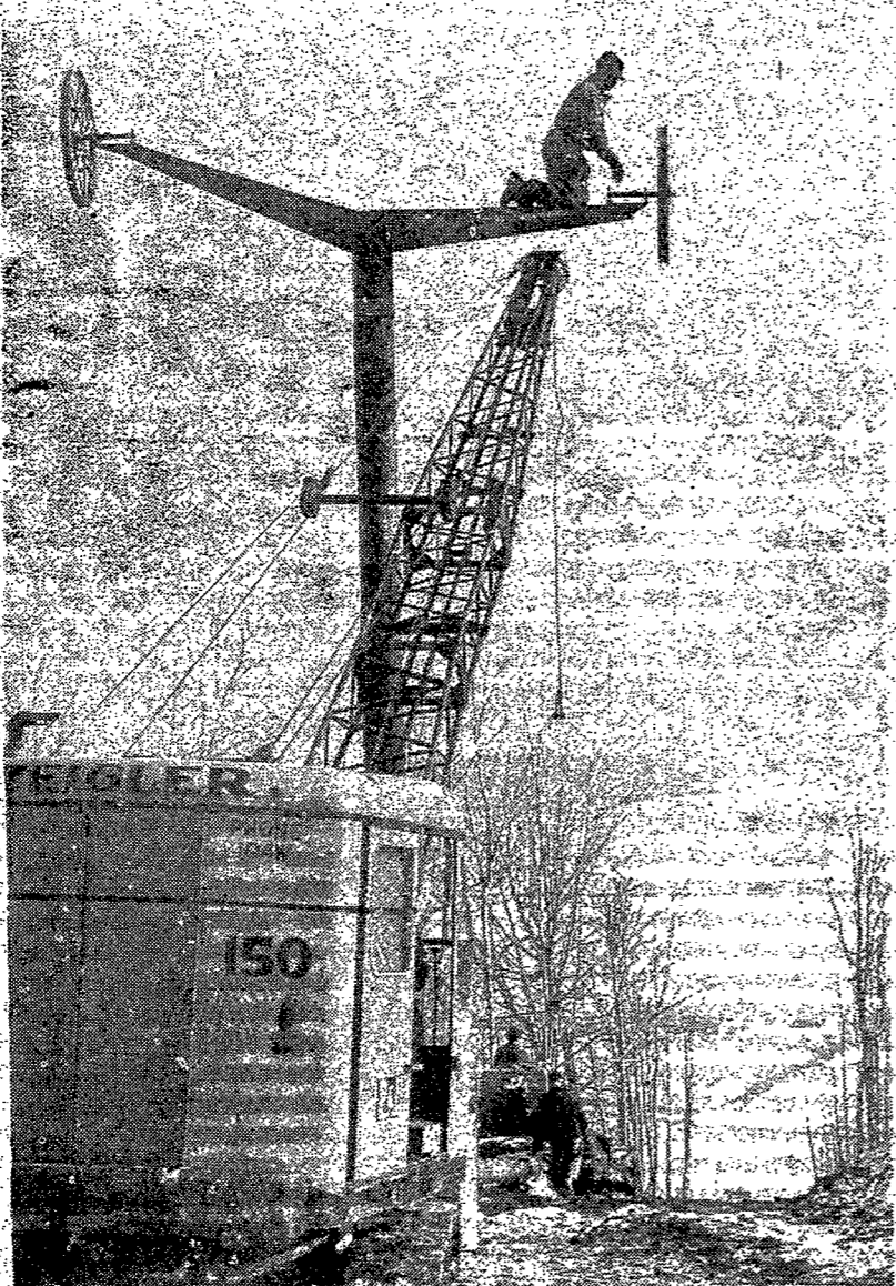
THE NEW POMAGALSKI LIFT at Snow Ridge is under operation now taking skiers at the popular Turin ski center to the top of No. 1 slope. The lift, shown above under construction, was imported from France. Skiers rest on a disk at the end of a long bar which hangs from the cable. The erection of the lift was done by a Syracuse engineer with local workmanship and labor. Photos through the courtesy of the Boonville Herald.
